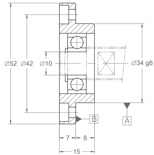
Section X-X
