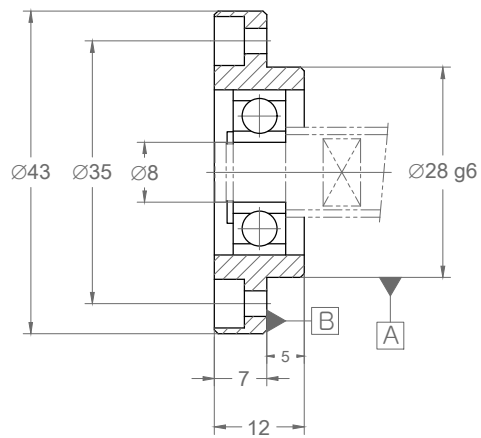
Section X-X
