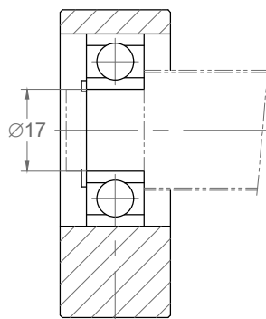
Section X-X
