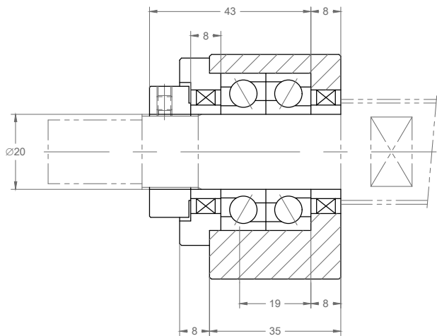
Section X-X
