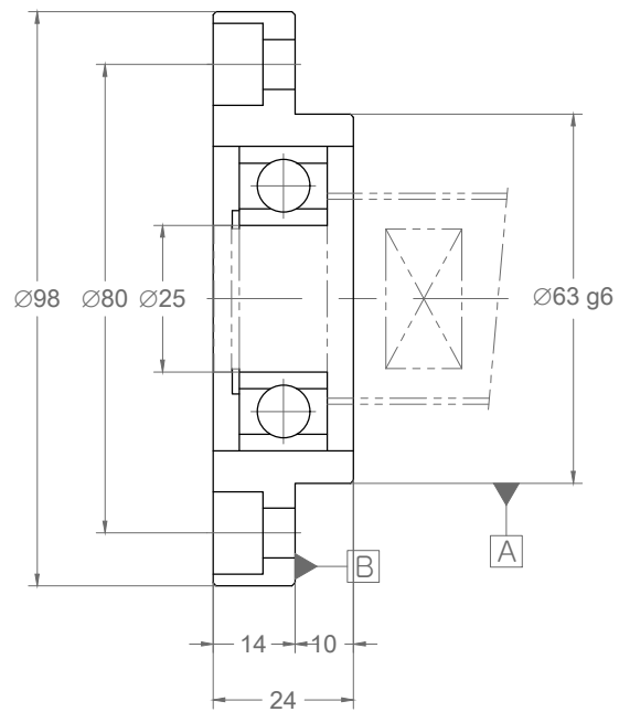
Section X-X
