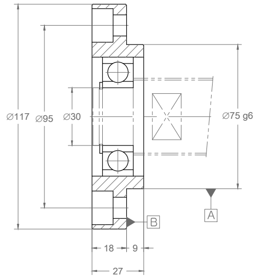
Section X-X
