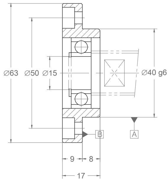
Section X-X
