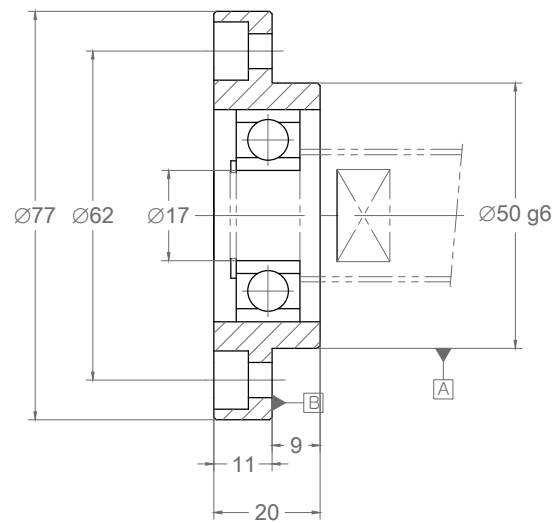
Section X-X
